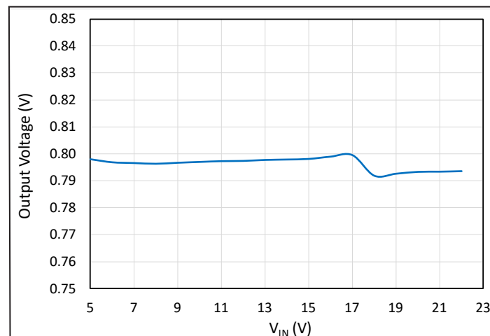
Figure 19. Line Regulation
