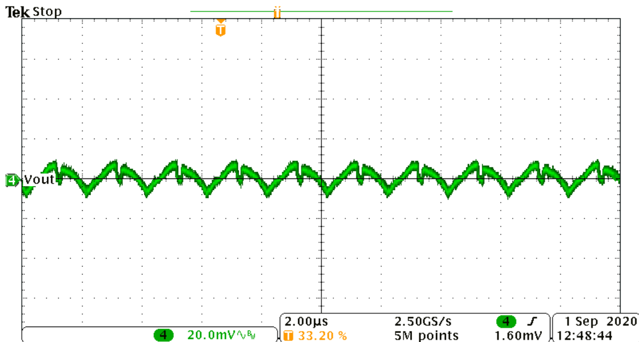
Figure 15: Channel 1 Output Voltage Ripple ( V_{IN} = 12V , V_{OUT} = 1.5V , Load = 25A)
