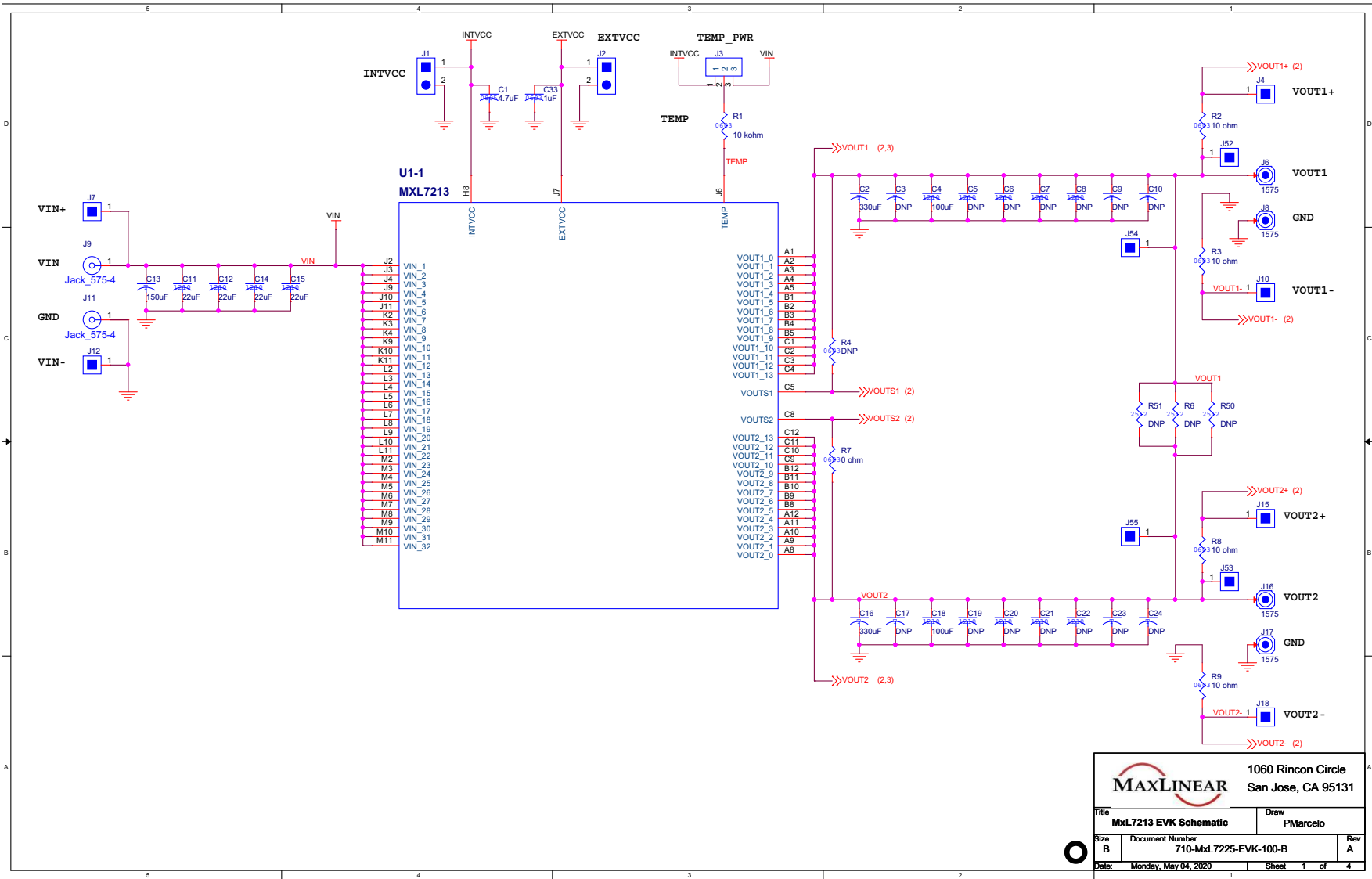
Figure 17: EVB Schematic
