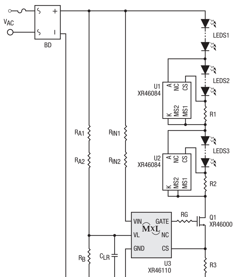
Figure 1. Typical Application
