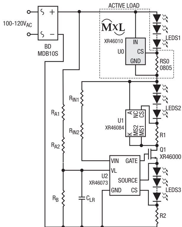
Figure 1. Typical Application
