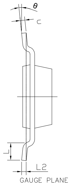
SIDE VIEW 1
