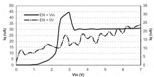
Fig. 7: I_q vs. V_{in} (fixed 3.0V, I_O=0\mu A )
