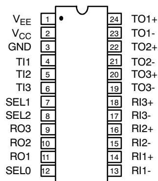
24 Lead PDIP (0.600")
