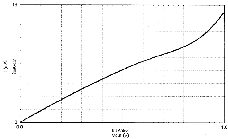
Figure 11. Output Sink Current vs. Output Voltage
