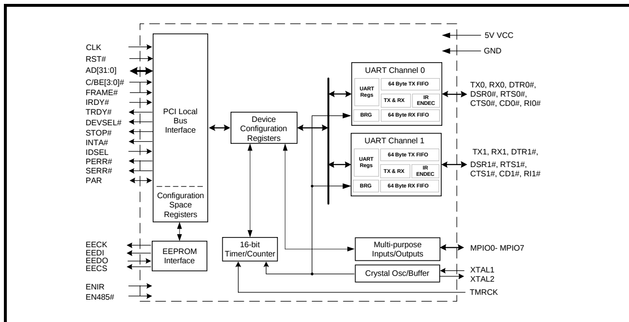
FIGURE 1. BLOCK DIAGRAM
