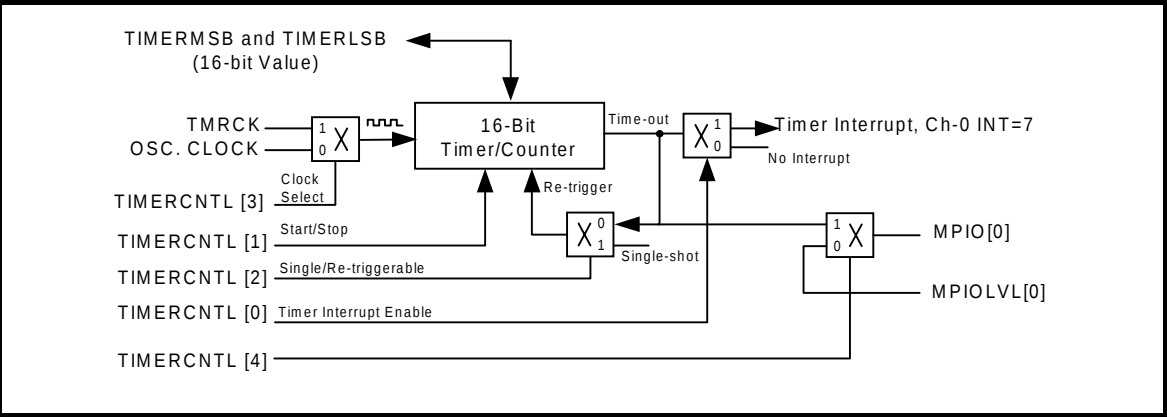
FIGURE 5. TIMER/COUNTER CIRCUIT.
