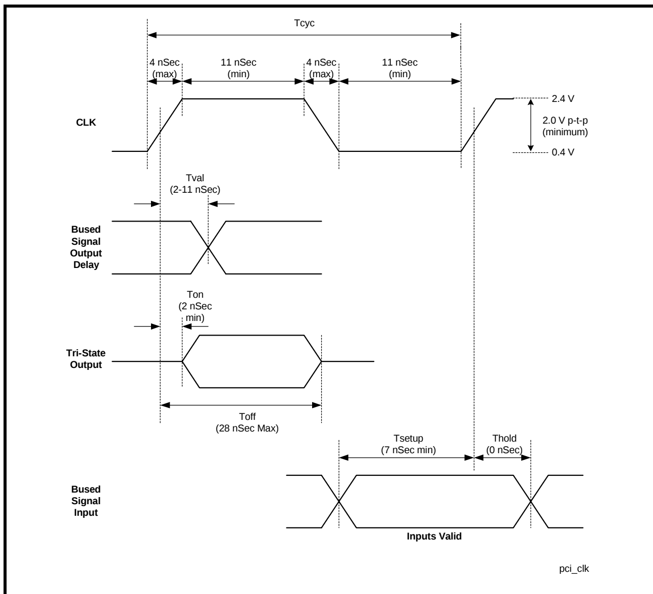
FIGURE 21. 5V PCI Bus Clock
