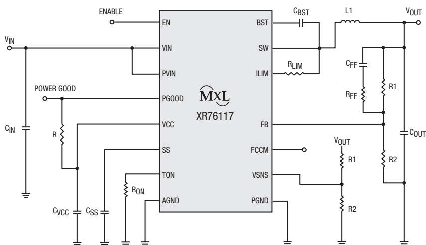
Figure 1. Typical Application
