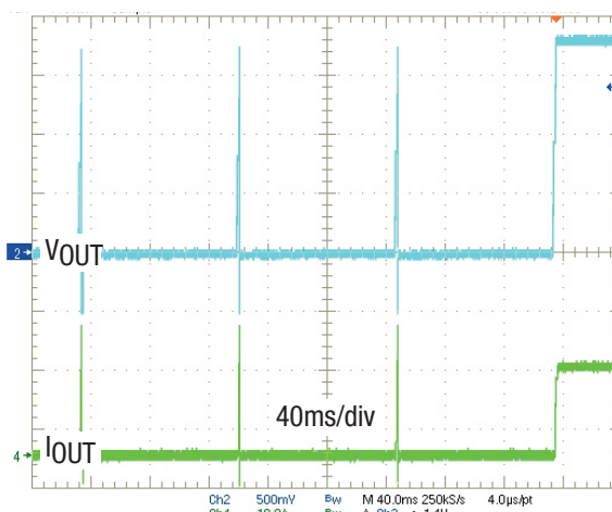
Figure 16. Short-Circuit Recovery, I_{OUT} = 15A
