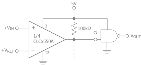
Figure 16. Driving CMOS
