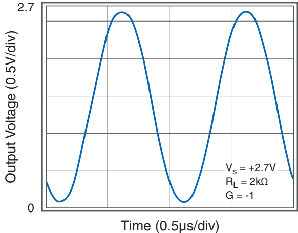
Output Swing
