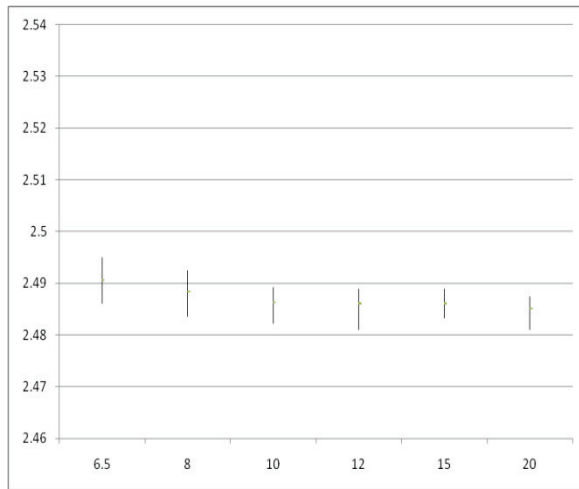
Figure 16: Line Load Regulation 2.5V
