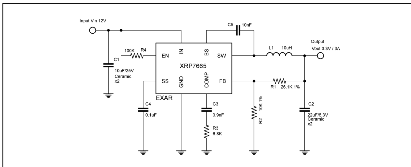
Fig. 1: XRP7665 Application Diagram
