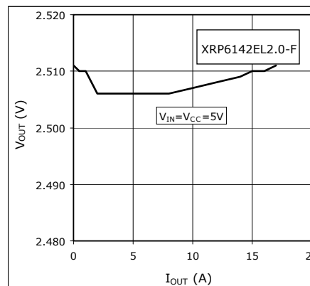
Fig. 7: Load regulation
