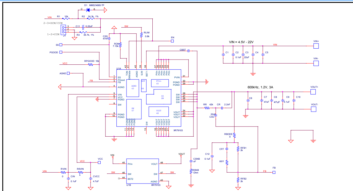
Fig. 1: XR79103 Evaluation Board Schematics
