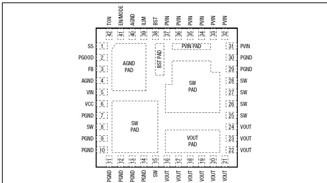
Fig. 2: XR79103 Pin Assignment
