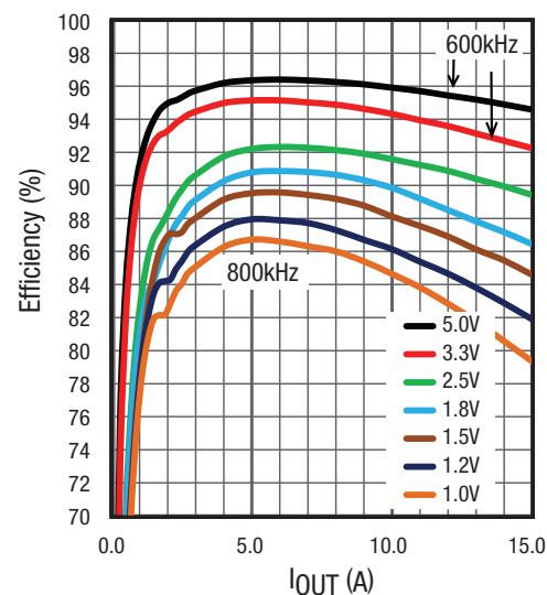
Figure 2. Efficiency
