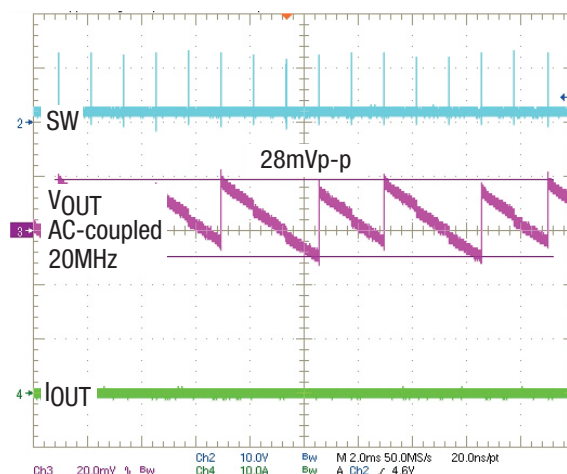
Figure 8. Steady State, DCM, I_{OUT} = 0A
