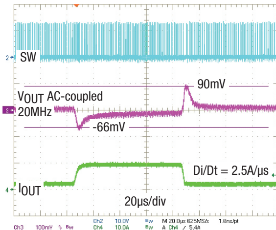
Figure 12. Load Transient, DCM, 2A to 9.5A
