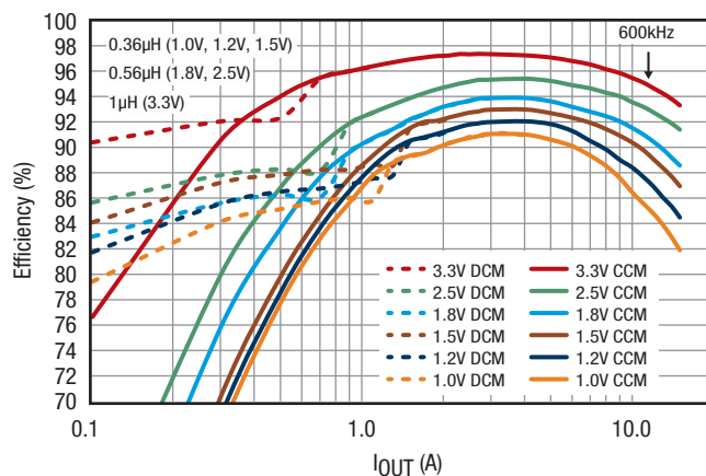
Figure 4. Efficiency, V_{\text{IN}} = 5\text{V}
