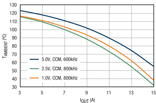
Figure 5. Maximum T_{\text{AMBIENT}} vs. I_{\text{OUT}} , V_{\text{IN}} = 12\text{V} , No Airflow
