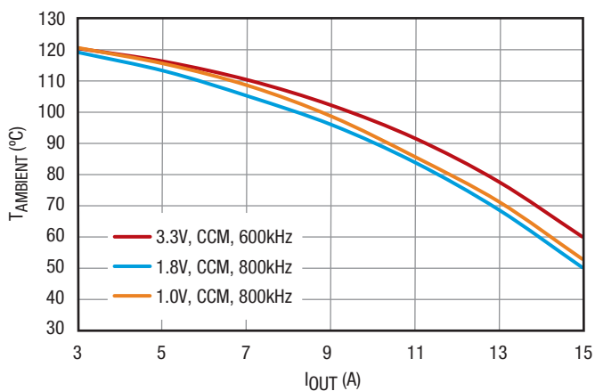
Figure 6. Maximum T_{\text{AMBIENT}} vs. I_{\text{OUT}} , V_{\text{IN}} = 5\text{V} , No Airflow
