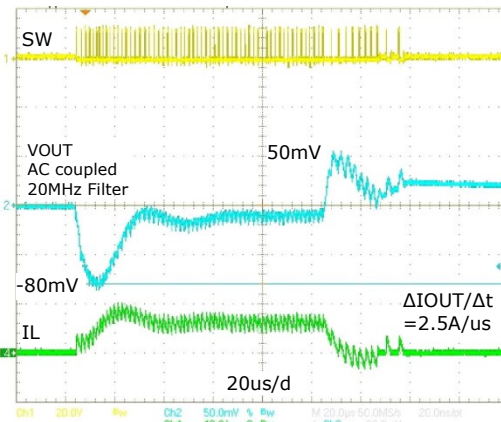
Figure 15: XR76112 Load Step, DCM / CCM, 0A - 6A - 0A
