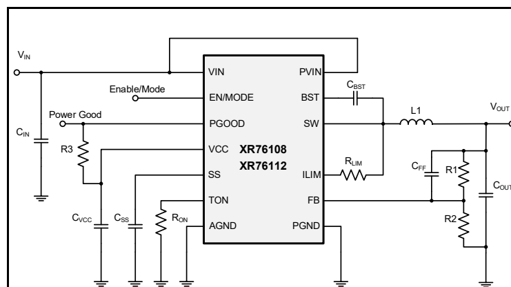
Figure 1: XR76108 and XR76112 Application Diagram
