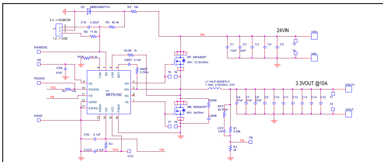
Fig. 1: XR75100 Evaluation Board Schematics
