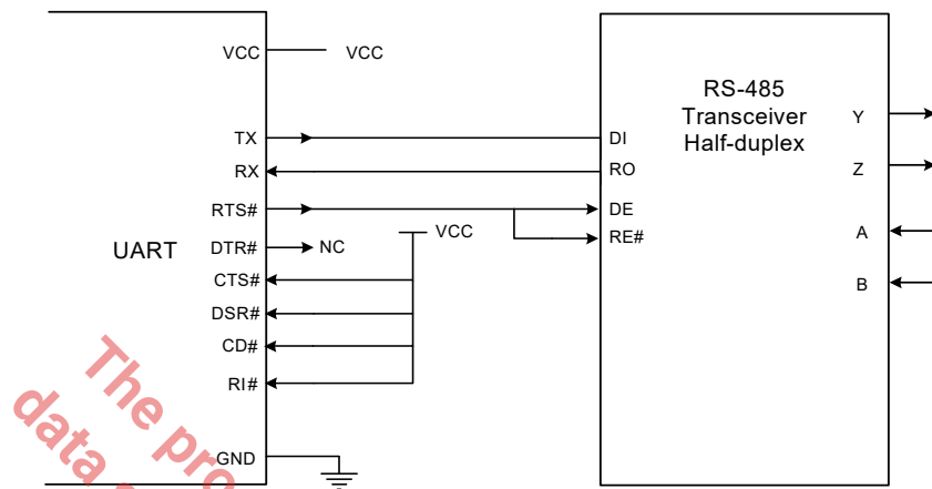
RS-485 Half-Duplex Serial Interface
