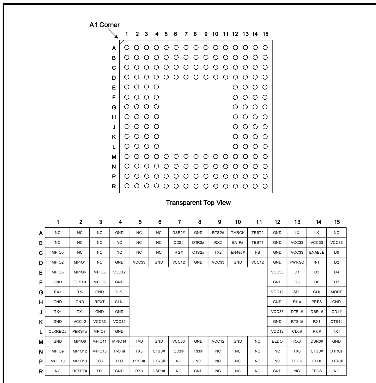
FIGURE 2. 176-FPBGA PINOUT
