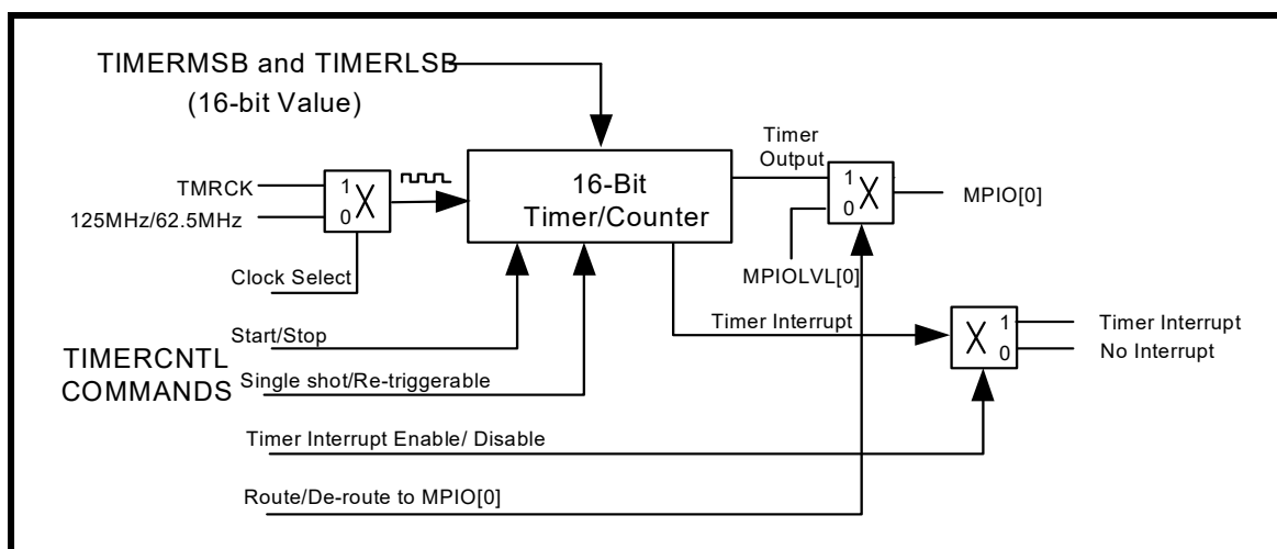
FIGURE 6. TIMER/COUNTER CIRCUIT
