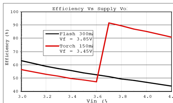
Fig. 15: Efficiency vs Supply Voltage D1=AOT3228HPW0303B LED, R_{SENSE}=0.3\Omega R_{SET}=140k\Omega , C_{IN}=2.2\mu F , C_{FC}=0.47\mu F , C_{OUT}=1\mu F
