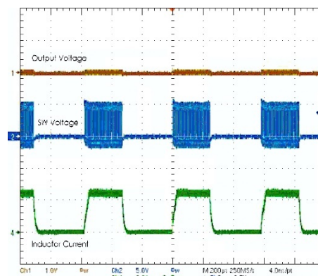
Fig. 19: Short Circuit Response
