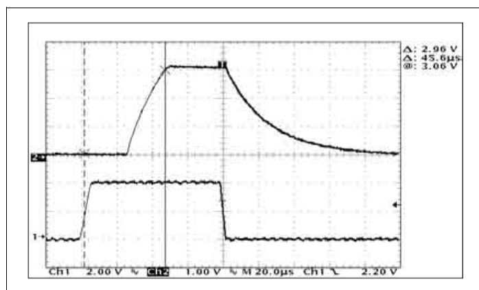
Figure 19: Turn-on Characteristic ( V_{IN} = 4V , I_{OUT} = 100mA )
