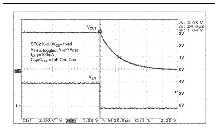
Figure 25: Turn-off Time ( V_{IN} = 7V , I_{OUT} = 100mA )
