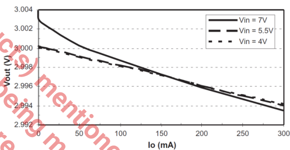
Fig. 19: Load Regulation (SP6201 fixed 3.0V)
