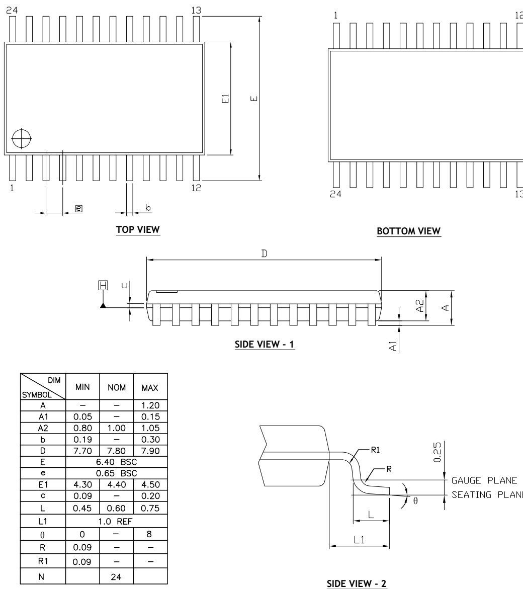
TERMINAL DETAILS
