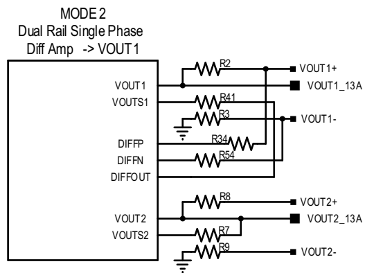
Figure 6: Mode 2 Block Diagram
