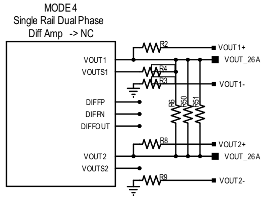
Figure 8: Mode 4 Block Diagram
