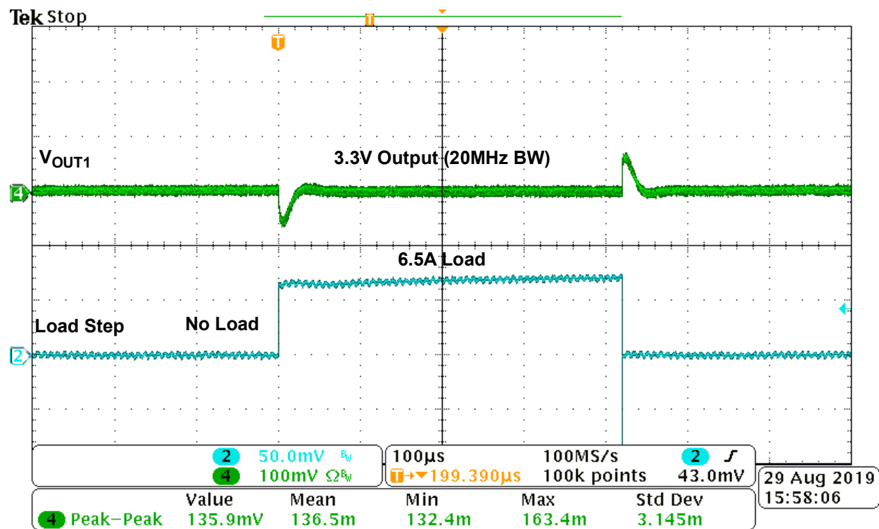
Figure 13: Channel 1 Load Transient Response ( V_{\text{OUT}} = 3.3\text{V} , V_{\text{IN}} = 12\text{V} )
