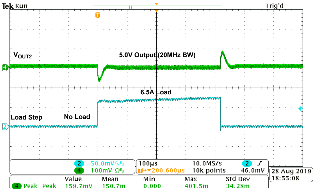
Figure 14: Channel 2 Load Transient Response ( V_{\text{OUT}} = 5.0\text{V} , V_{\text{IN}} = 12\text{V} )
