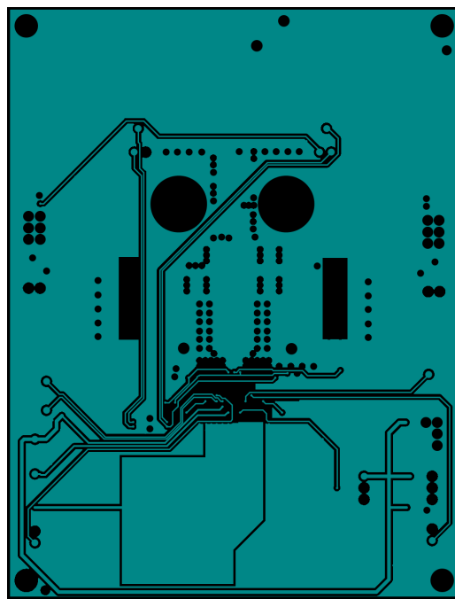
Figure 25: EVB PCB Layer 5
