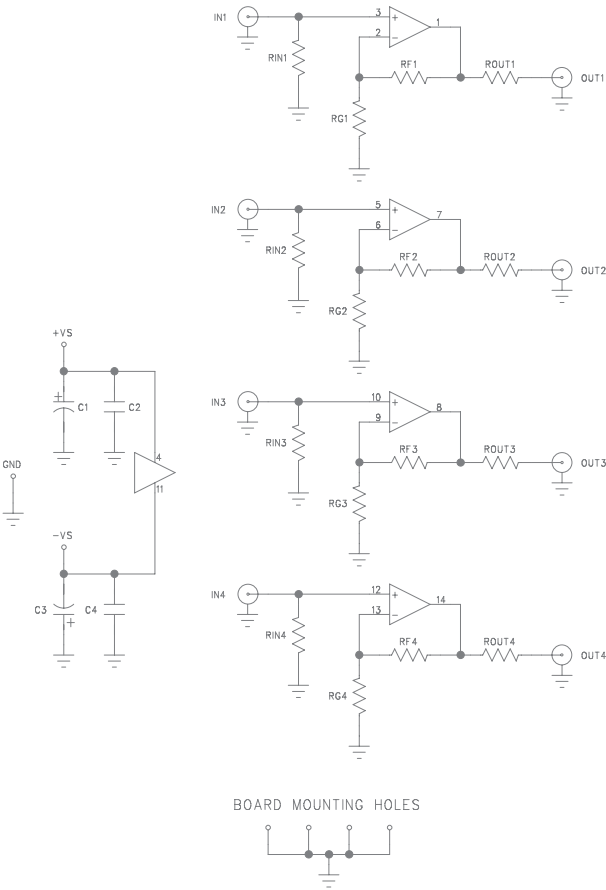
Figure 10. CEB018 Schematic
