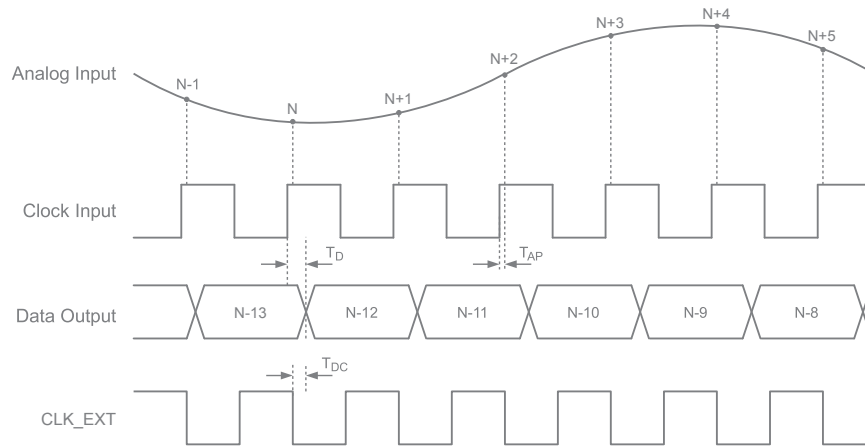
Figure 1. Timing Diagram
