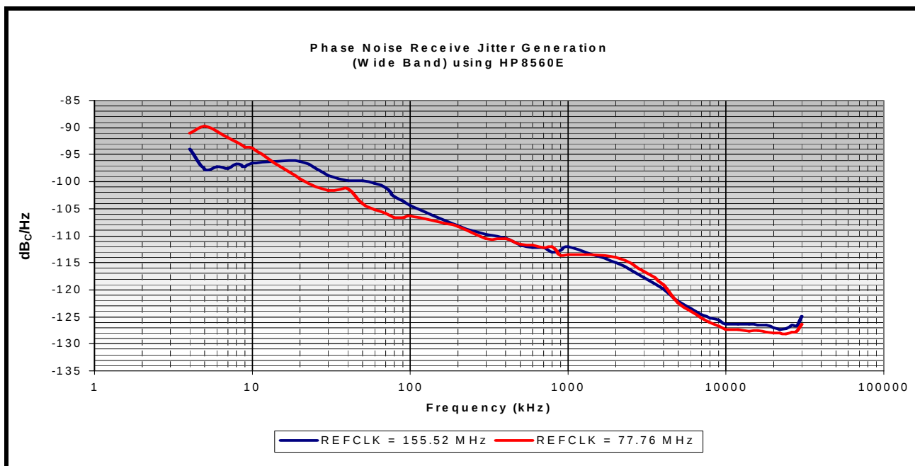
FIGURE 25. 91L80 MEASURED ELECTRICAL PHASE NOISE RECEIVE JITTER GENERATION AT 2.488 GBPS
