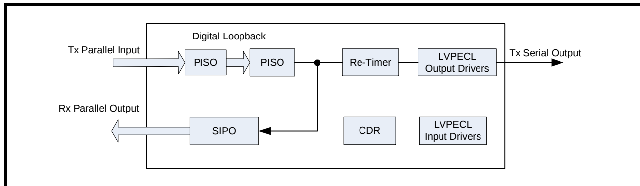
FIGURE 18. DIGITAL LOOPBACK
