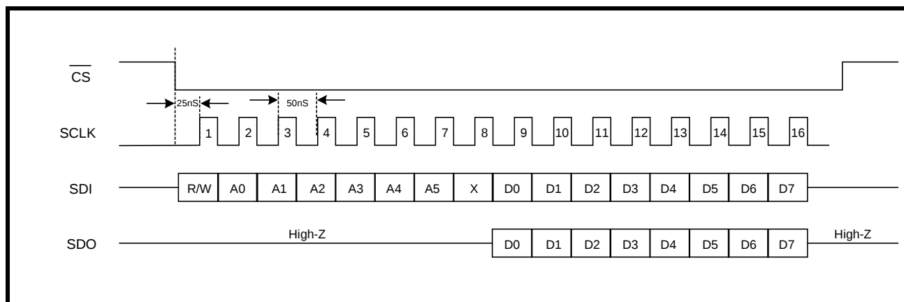
FIGURE 25. TIMING DIAGRAM FOR THE SERIAL MICROPROCESSOR INTERFACE
