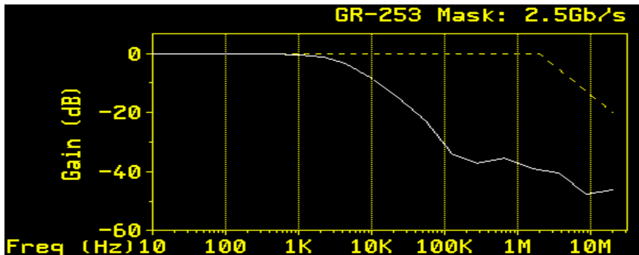
FIGURE 22. 91L80 MEASURED JITTER TRANSFER WITH EXTERNAL JITTER ATTENUATION ENABLED IN LOOPTIMING AT 2.488 GBPS IN STS-48.
