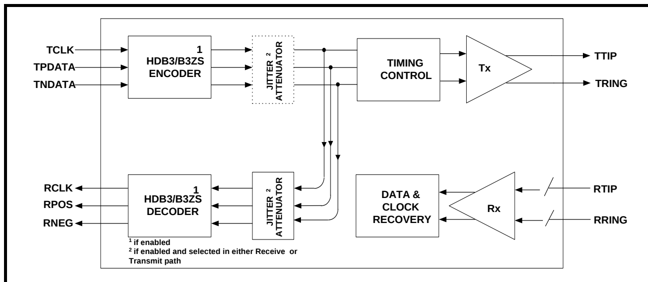
FIGURE 28. DIGITAL LOOPBACK
