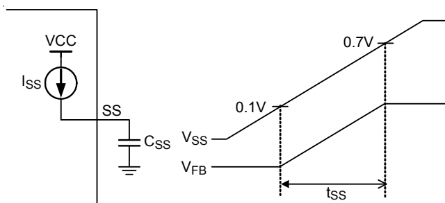
Figure 1. External Soft-Start Time Setting
