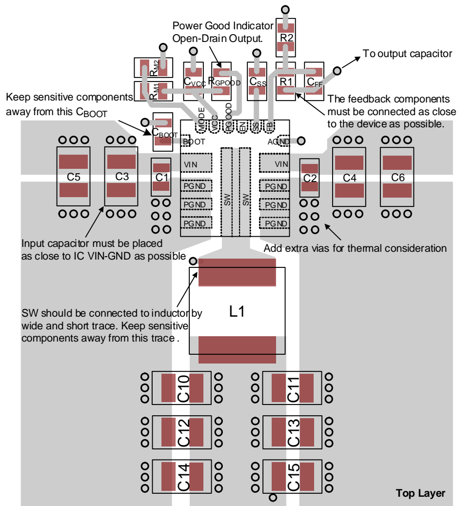
Figure 16. Layout Guide (Top Layer)
