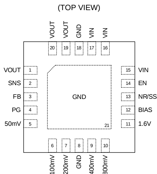
VQFN-20L 5x5
