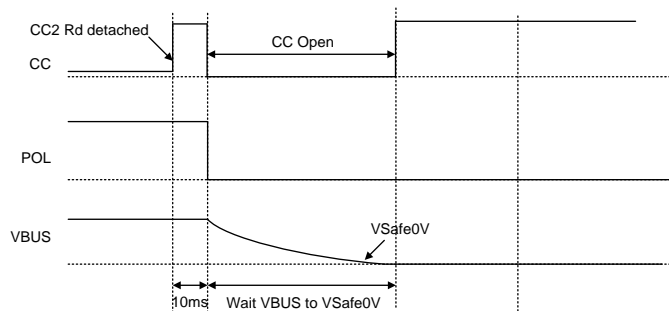
Figure 10. Type-C Detached Sequence
