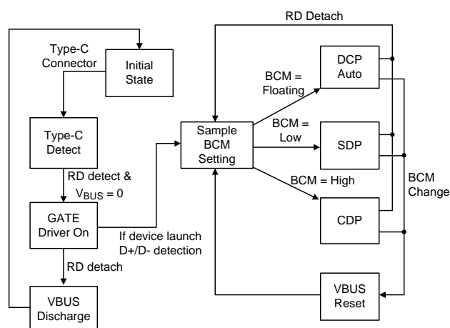
Figure 26. Detection Flow
