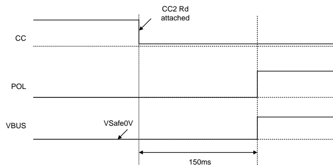
Figure 9. Type-C Attached Sequence
