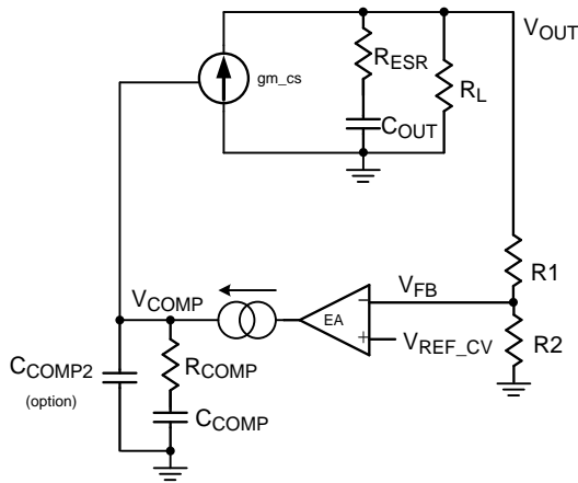
Figure 16. Simplified Equivalent Circuit of Buck with PCCM
