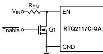
Figure 22. Logic Control for the EN Pin
