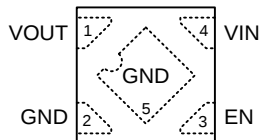
ZQFN-4L 1x1
