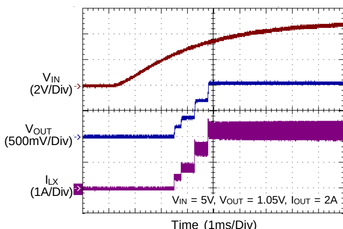
Figure 2. Soft-Start
