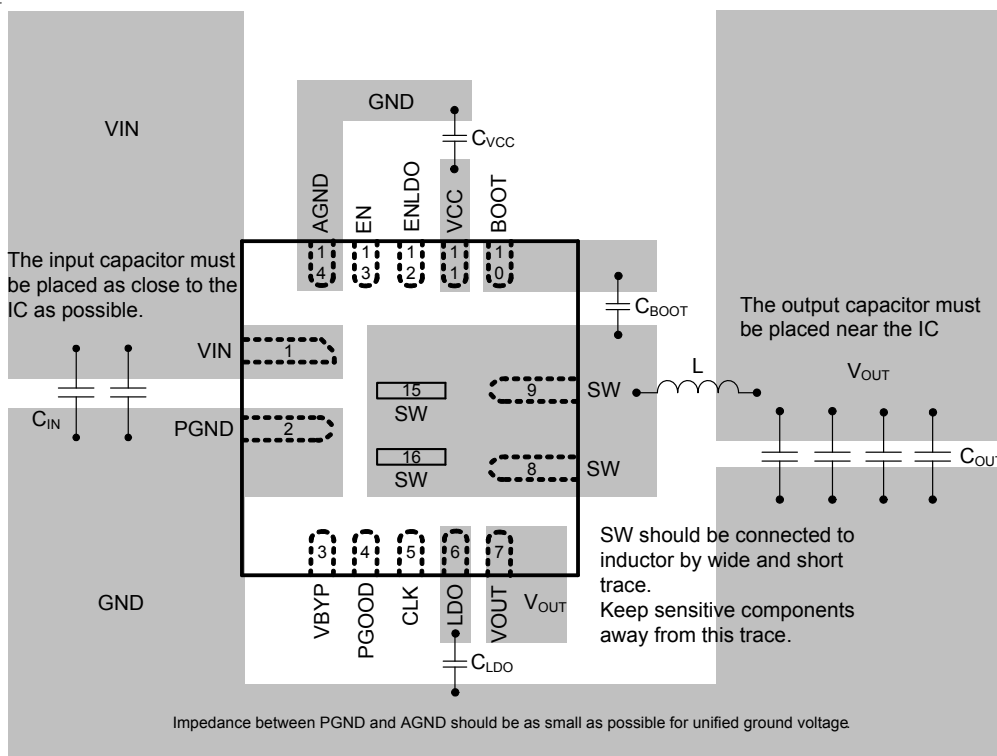
Figure 4. Layout Guide
