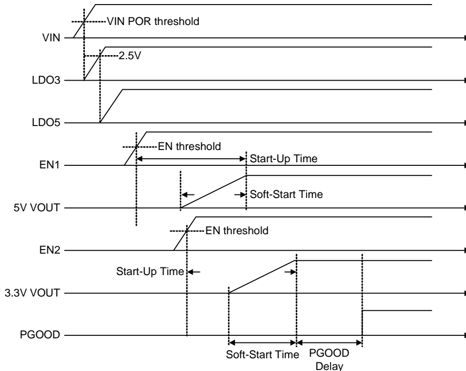
Figure 6. RT6575B Timing
