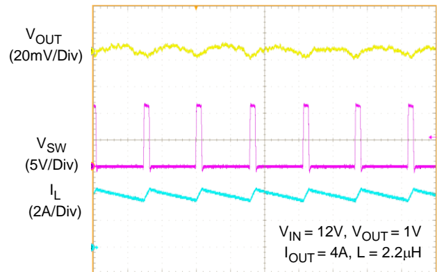
Output Ripple as IOUT = 4A
