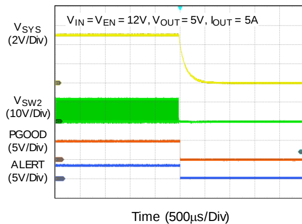
Reverse Power Off from I2C
