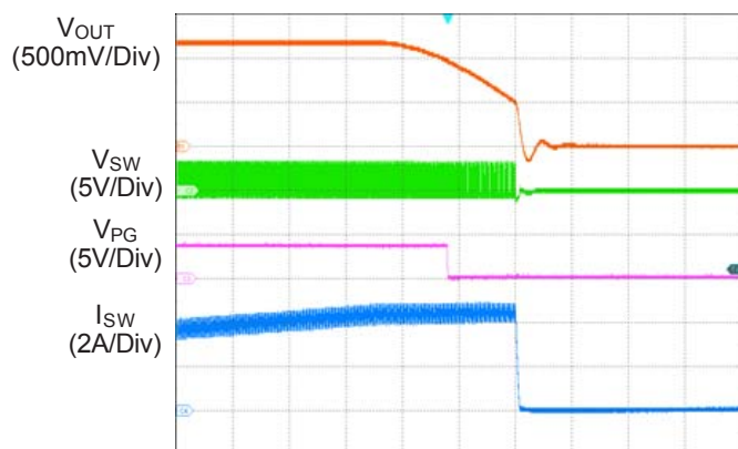
Figure 2. Over-Current Protection
