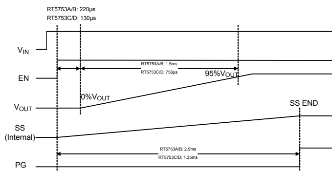
Figure 1. Start-Up Sequence
