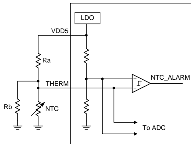
Figure 3. External Temperature Sense Circuit
