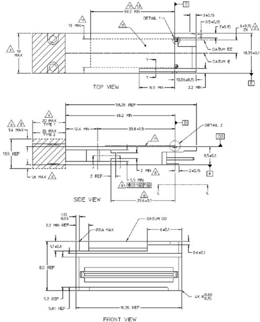
Figure 2. FTCD8613E2PCM Mechanical Dimensions.
