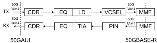
Figure 2. Duplex 50G Transceiver Architecture
