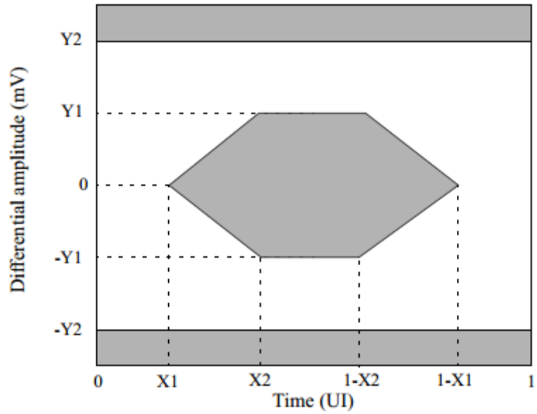
Figure 2 – Transmitter Input Differential Signal Mask
