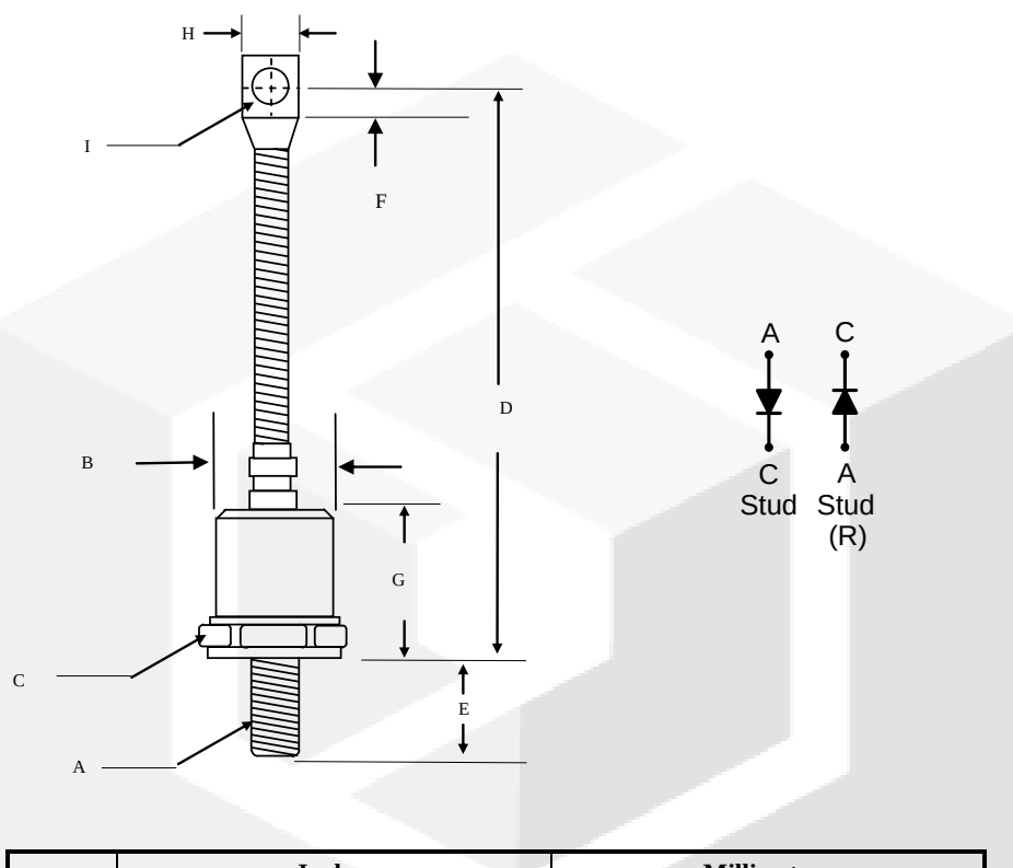
DO-8 (DO-205AA)
