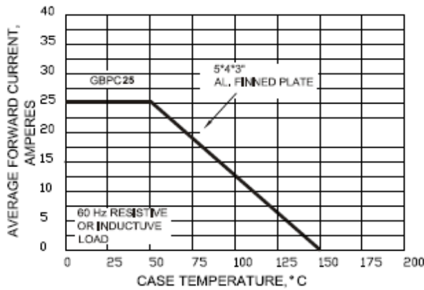
FIG.1-MAXIMUM OUTPUT RECTIFIED CURRENT
