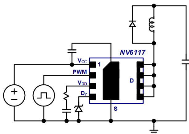
Fig. 1. Inductive switching circuit
